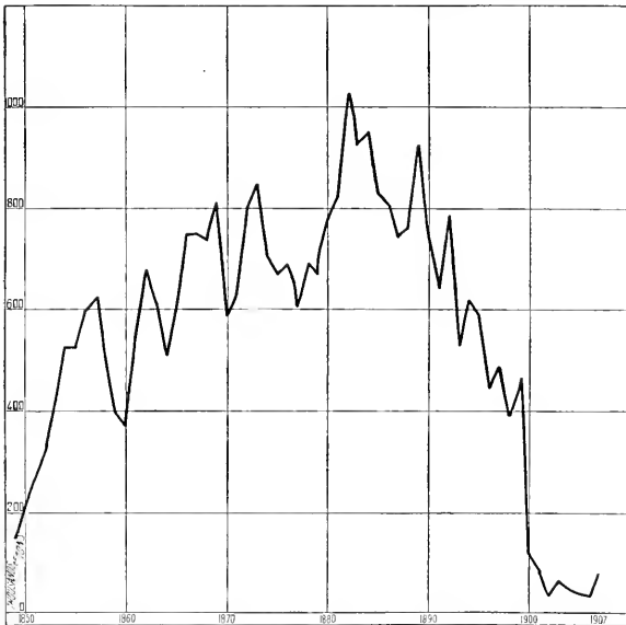
FIG. 42. Graph showing tons transported on Illinois and Michigan Canal from 1849 to 1907.
